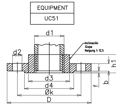
DETAILS FLANGES THREADED NECK
